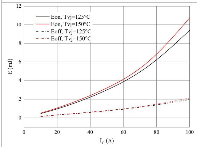
图 5. 开关损耗 Figure 5. Switching losses of IGBT V_{GE}=\pm 15V, R_{Gon}=8\Omega, R_{Goff}=8\Omega, V_{CE}=400V
