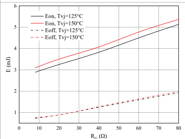
图 6. 开关损耗 Figure 6. Switching losses of IGBT V_{GE}=\pm 15V, I_C=50A, V_{CE}=400V
